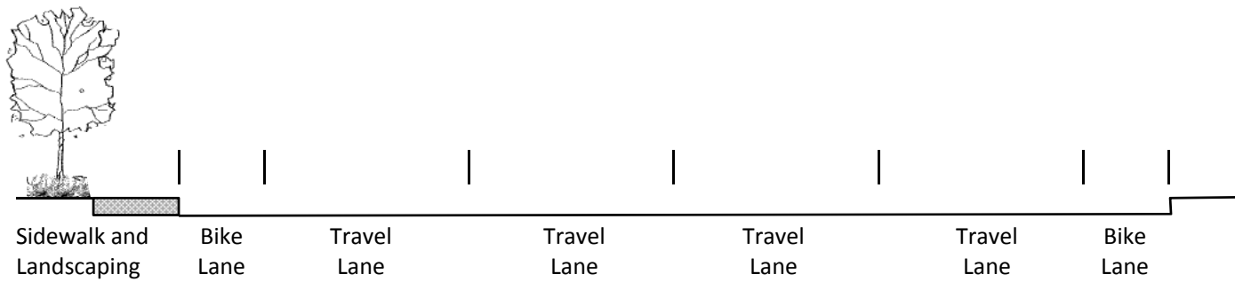
Typical Section – Air Cargo Road
